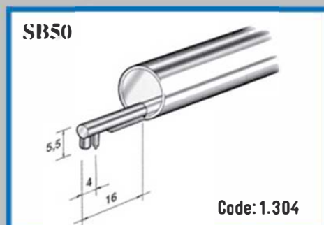
SB50 - With anterior skid, for plane or curve surfaces, ideal for measuring at 90°.
